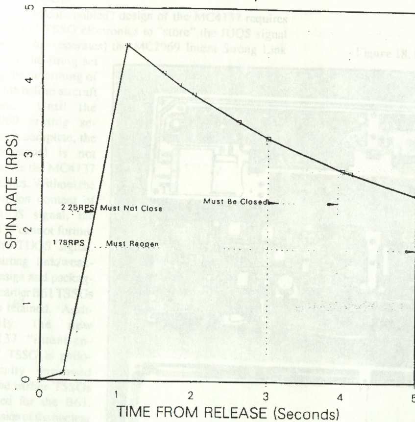
Figure 16. Functional Requirements for the Spin-sensing Rolamites, Minimum Spin Rate
